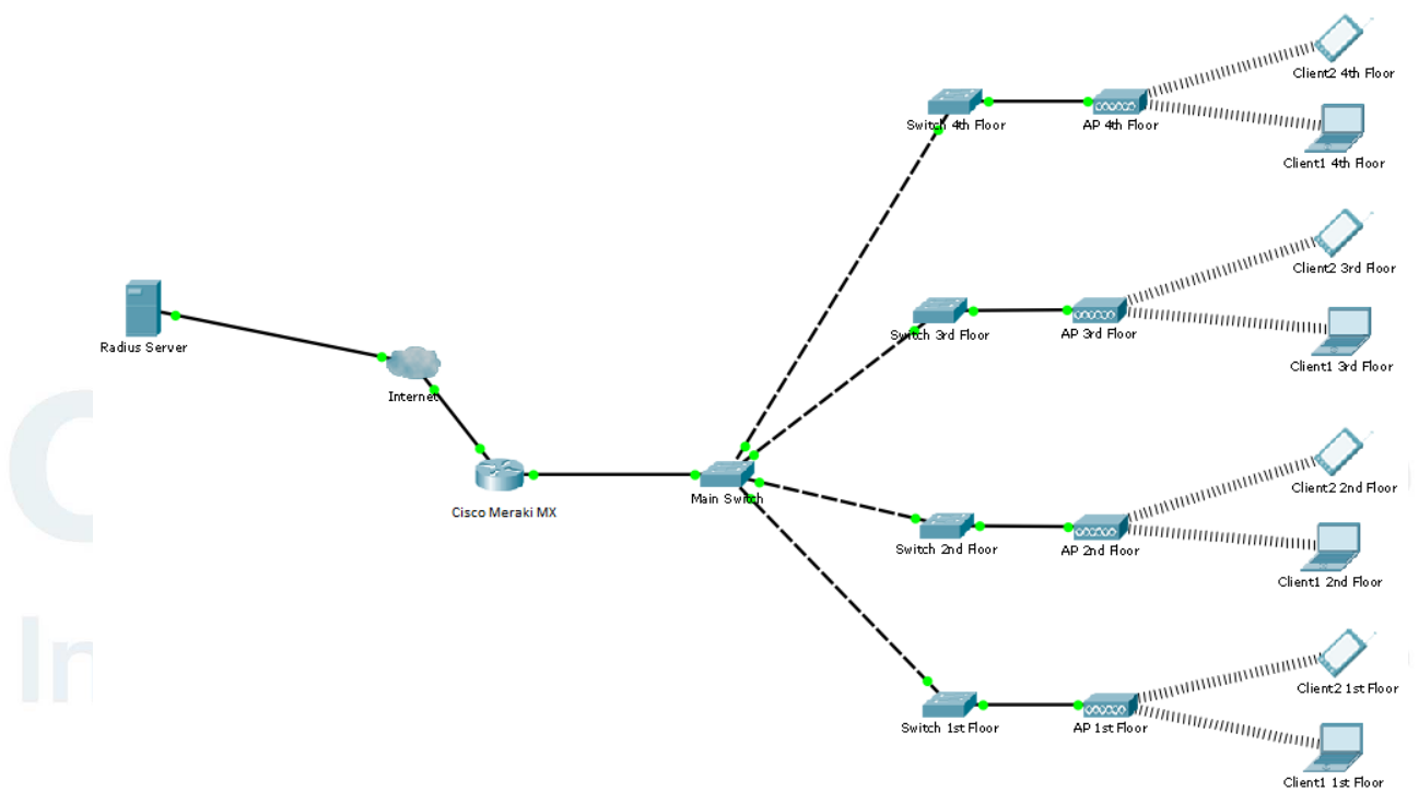
Basic Installation Topology for CHS
